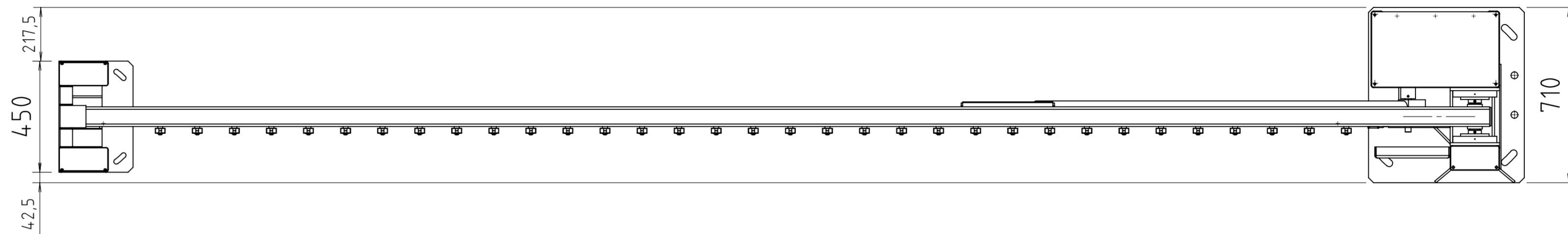
TOP VIEW GATE
